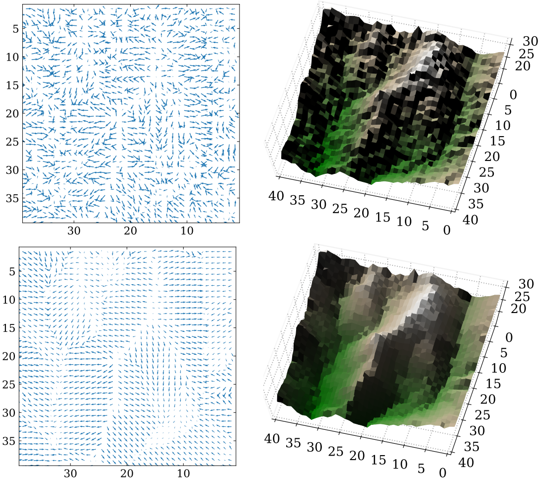
Figure 4.8: Denoising of \mathbb{S}^2 -valued surface normals on the digital elevation model (DEM) dataset from [Ges+09] ( noisy input on top ). The total variation model ( \lambda = 0.4 ) enforces flat hillsides in the denoised image ( bottom ). See Fig. 4.9 for results from Huber and quadratic regularization.
